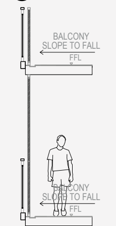
4 DETAIL "D1"
